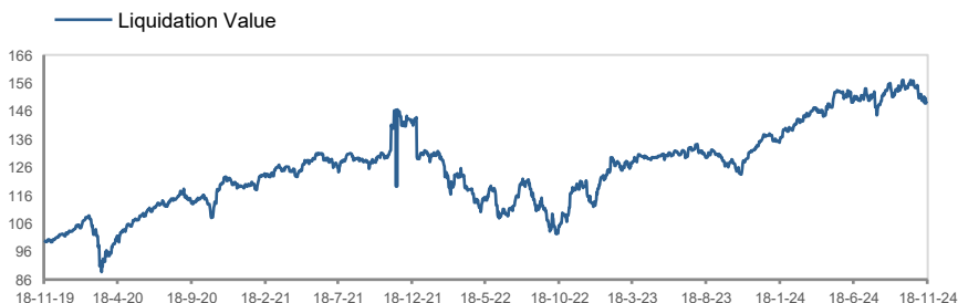
Cumulative returns 2019/11/18 a 2024/11/18
